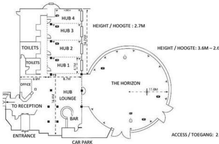
GROUND FLOOR / BEGANE GROND
